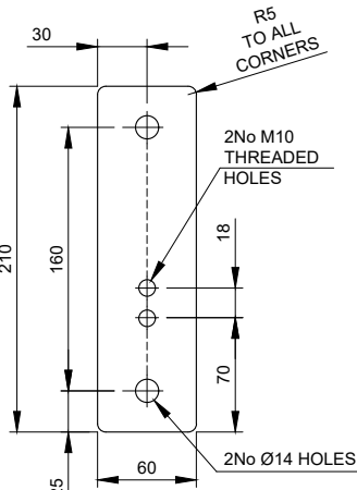
PART TPS-R Scale 1:5
