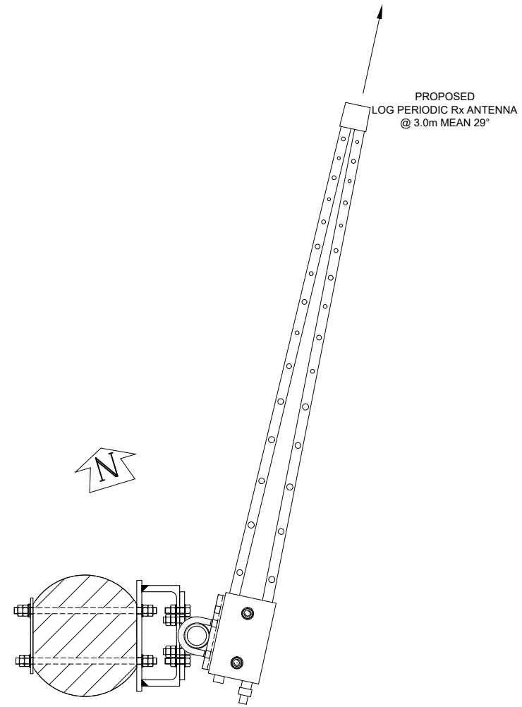
VIEW C-C Scale 1:10
