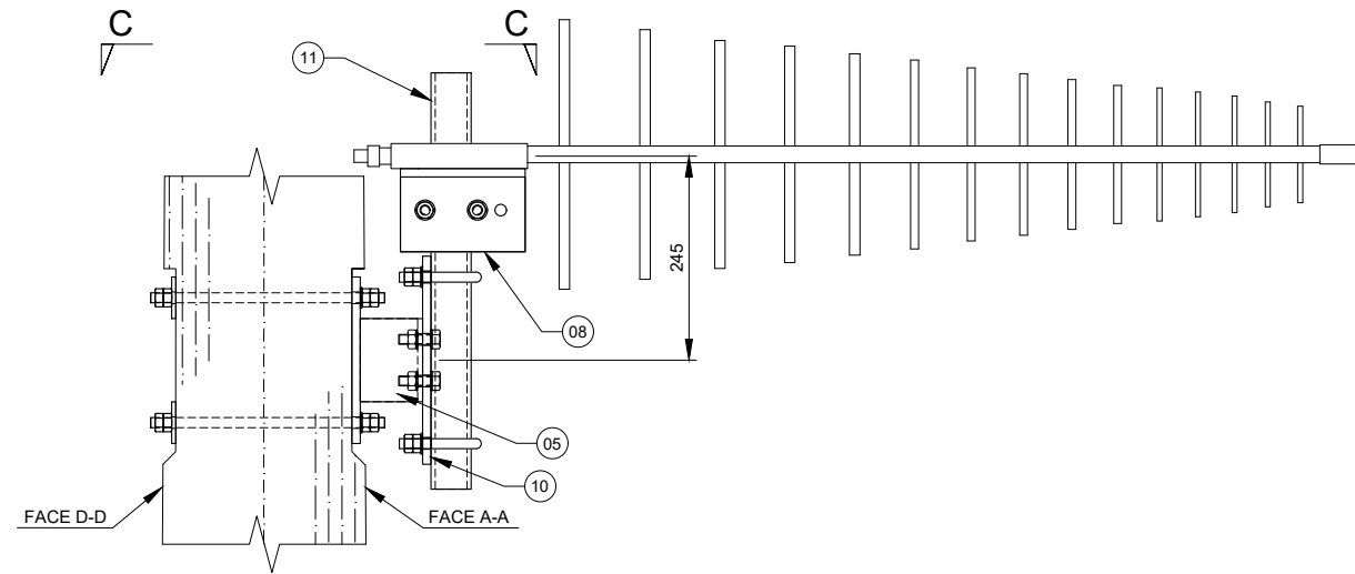
DETAIL H - Rx ANTENNA MOUNT Scale 1:10
